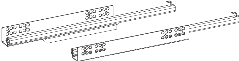
K 4 x 201030105 QUADRO 400
